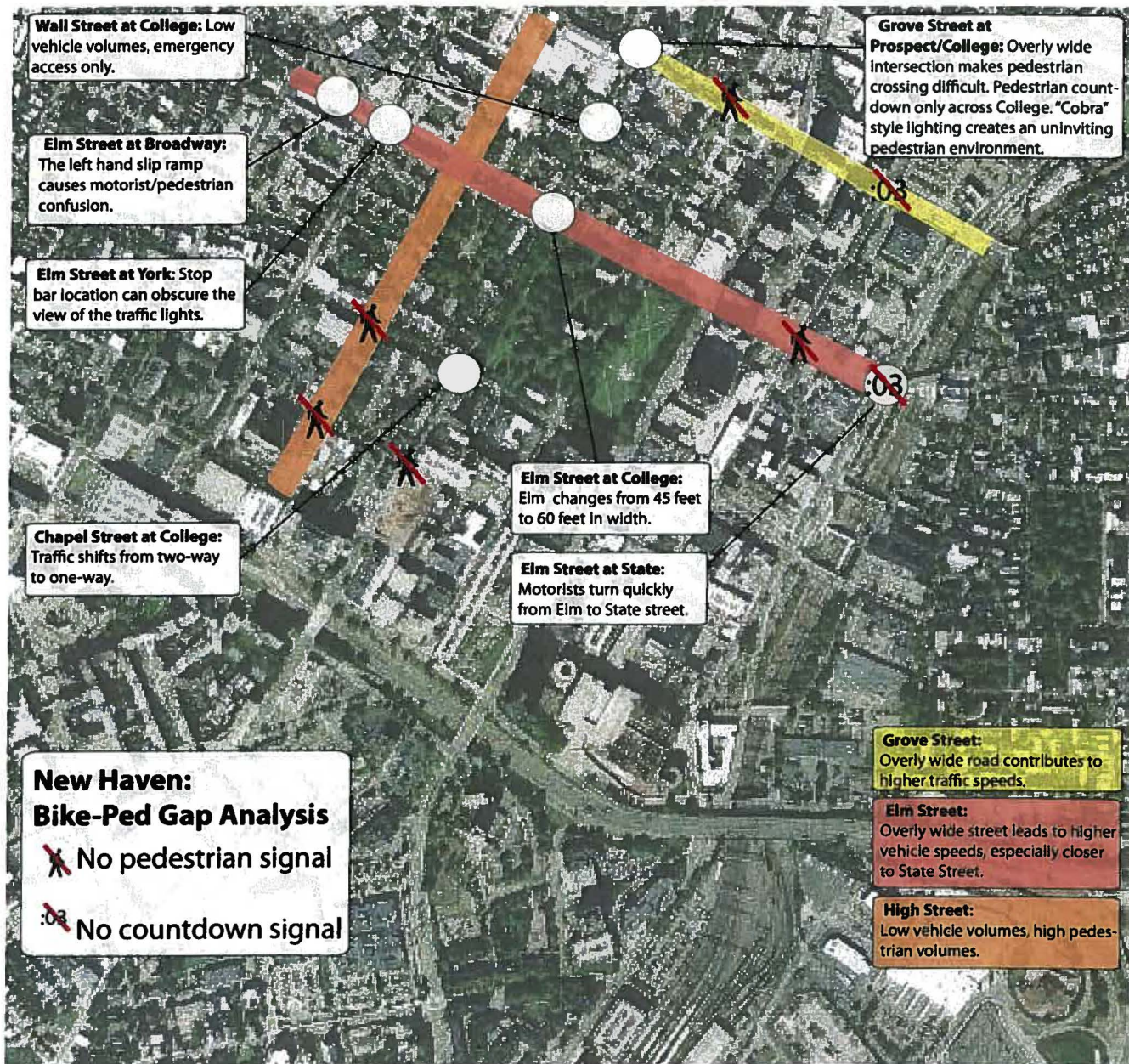
Figure 11: Existing Conditions
