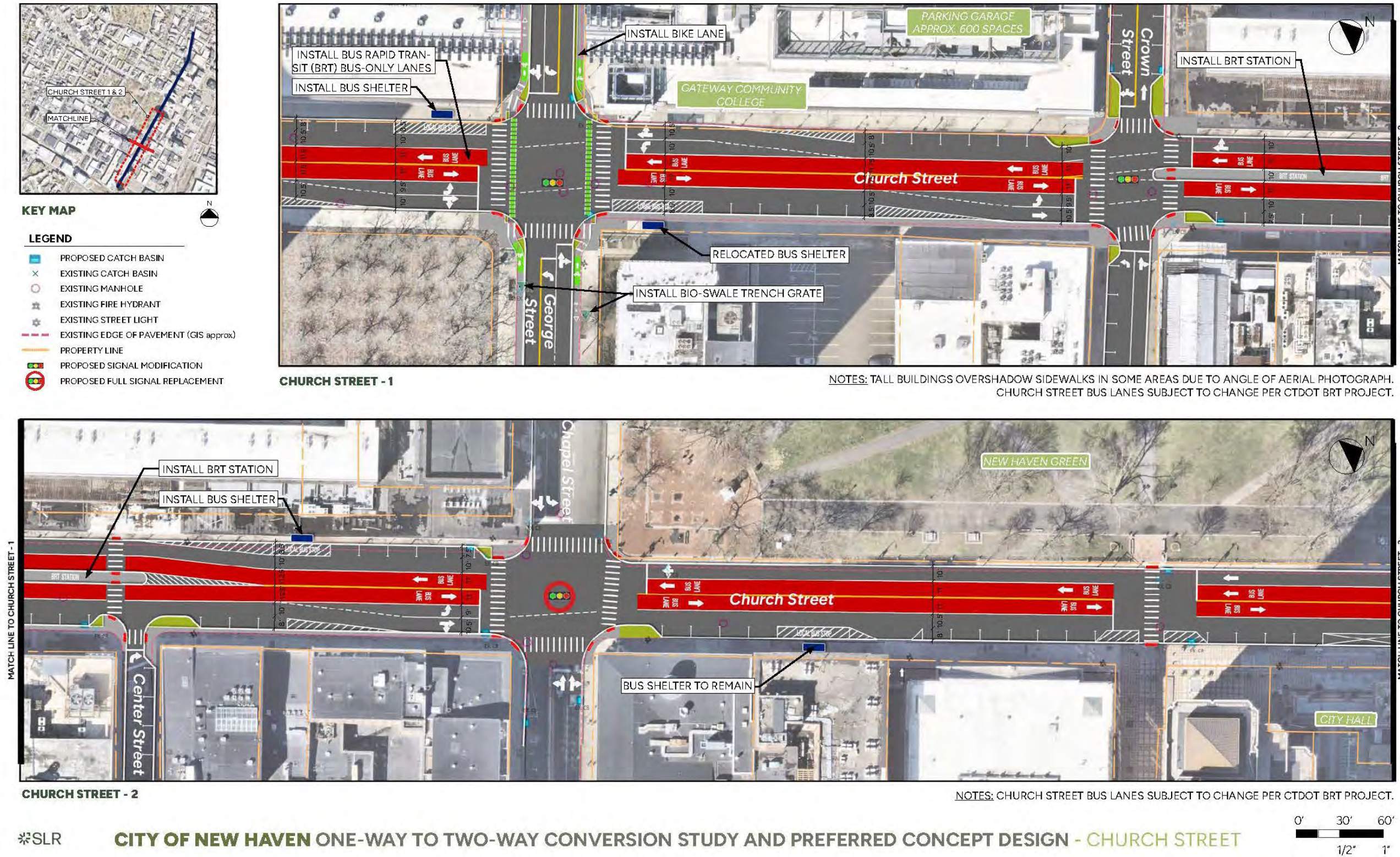
Figure 5.1 Two-Way Conversion Preferred Design – Church Street
