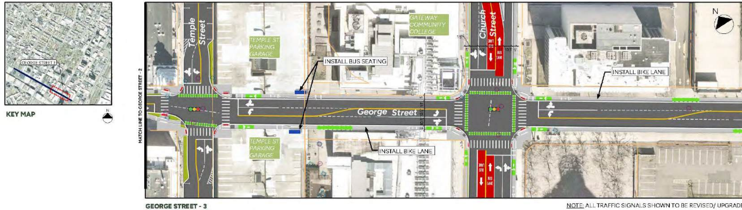
Figure 4.12 Two-Way Conversion Concept Design – George Street
