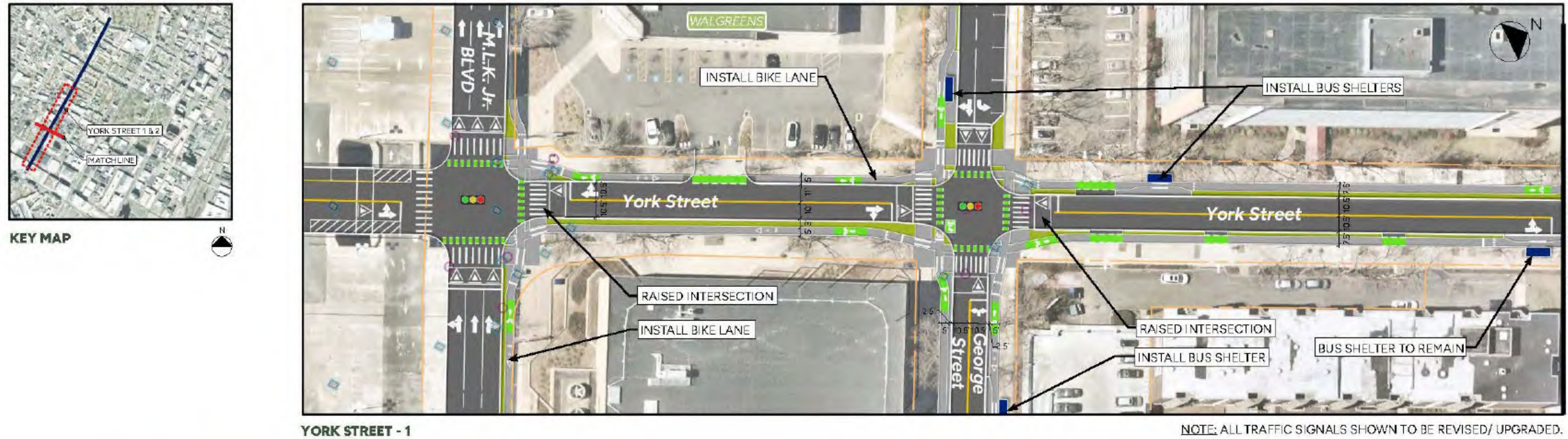
Figure 4.7 Two-Way Conversion Concept Design – York Street - Alternate 2
