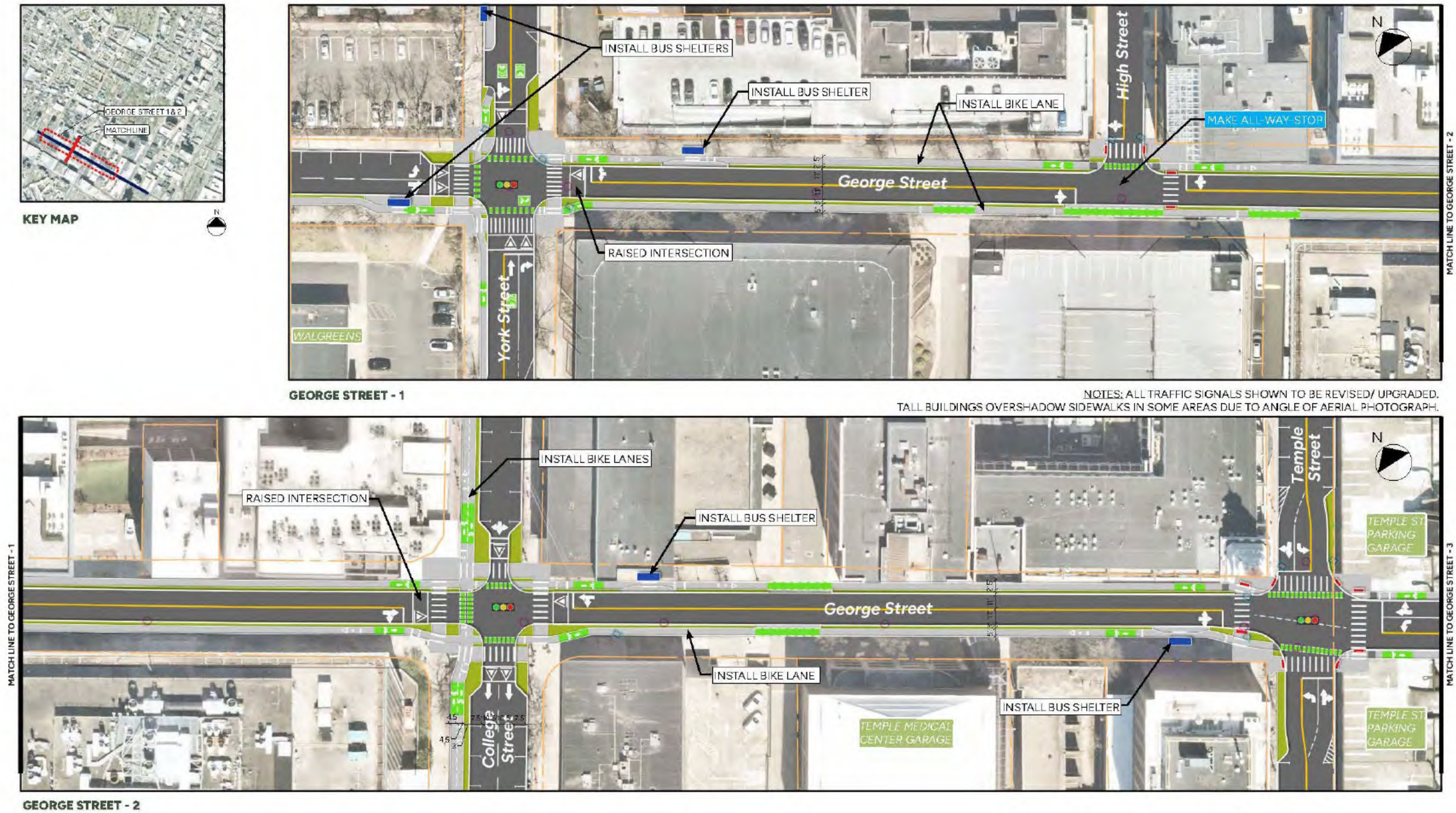
Figure 4.11 Two-Way Conversion Concept Design – George Street
