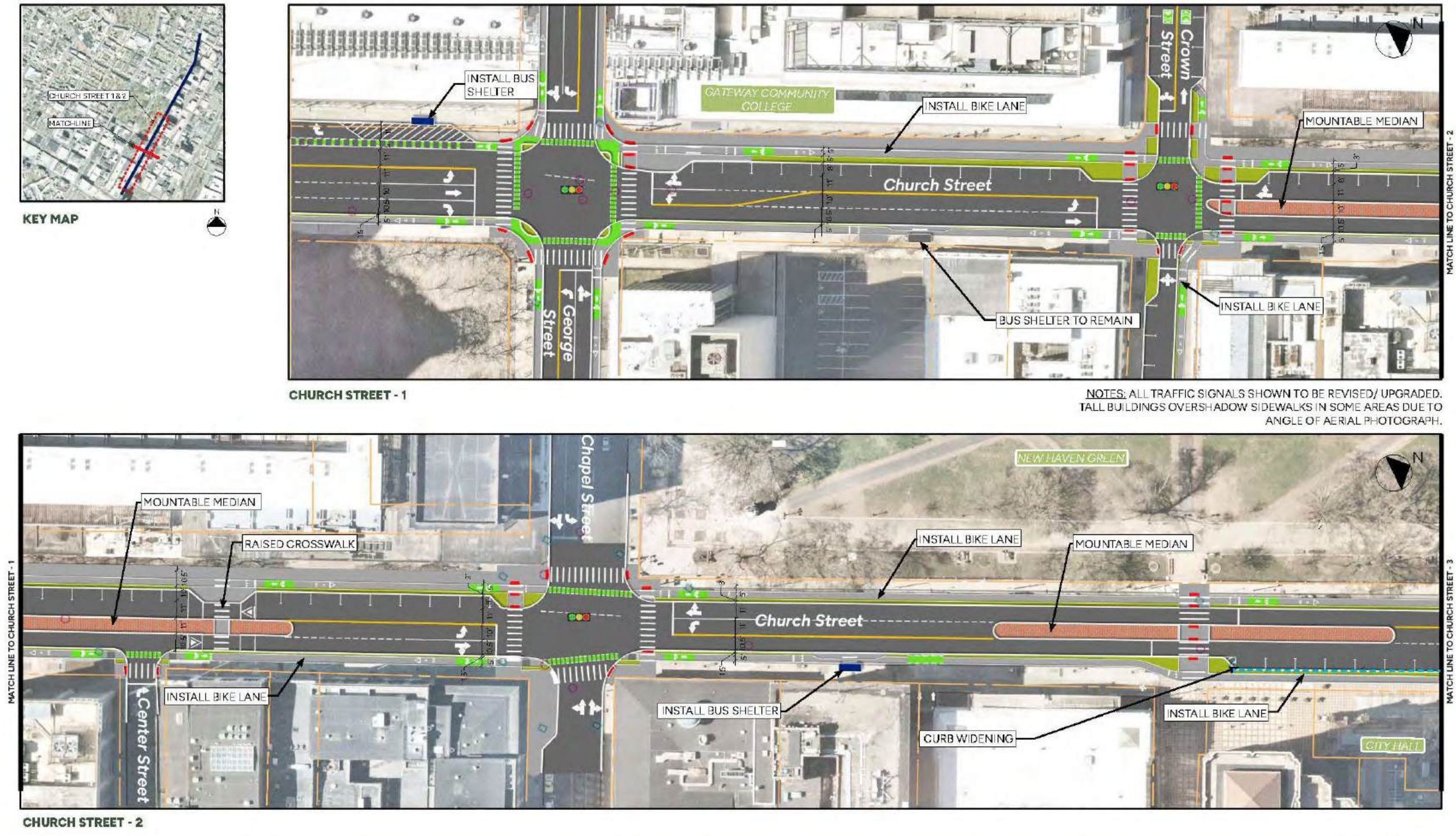
Figure 4.3 Two-Way Conversion Concept Design – Church Street - Alternate 2
