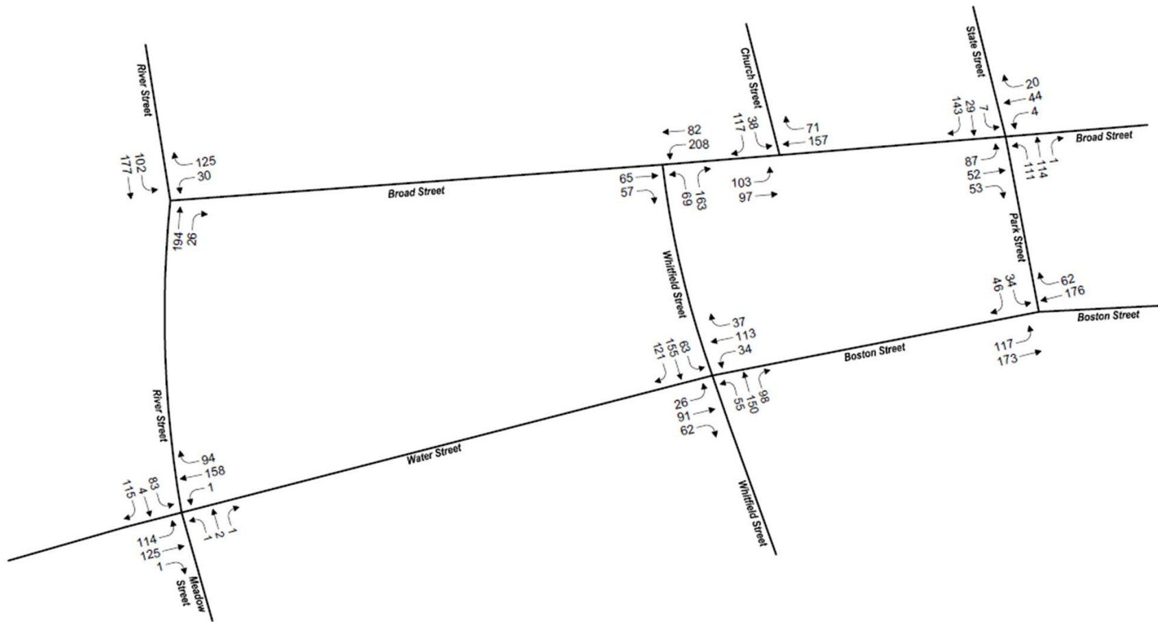
Figure 3 Existing Weekday PM Peak Traffic Volumes– Primary Study Area
