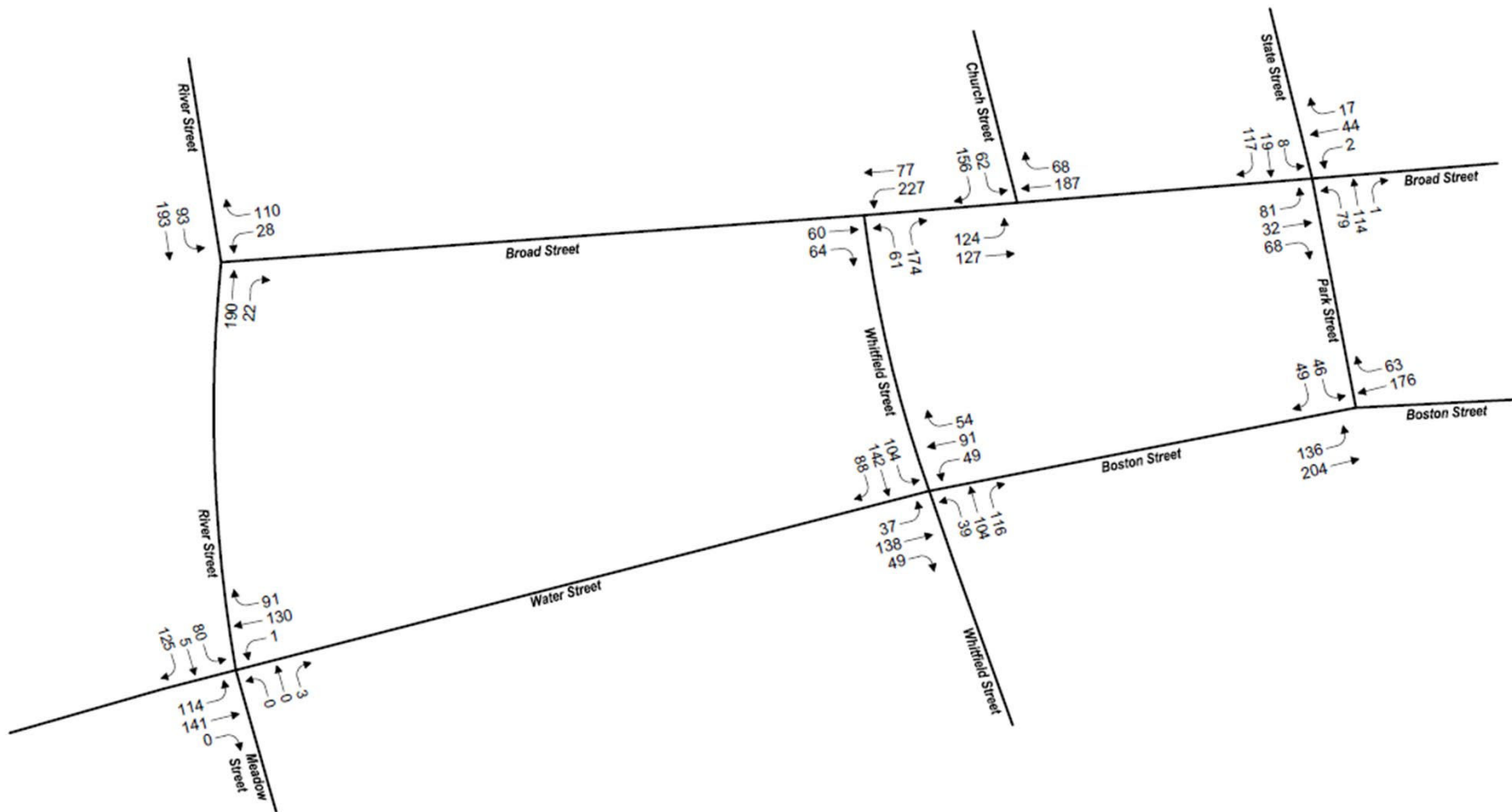
Figure 4 Existing Saturday Peak Traffic Volumes– Primary Study Area
