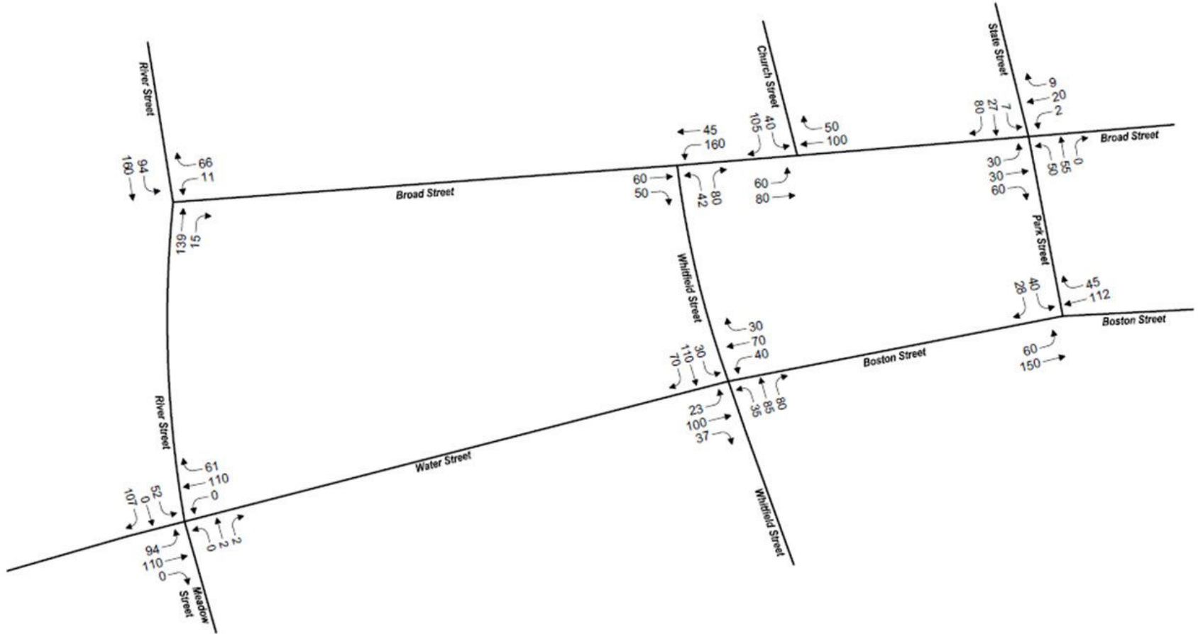
Figure 28 2029 No-Build AM Peak Traffic Volumes
