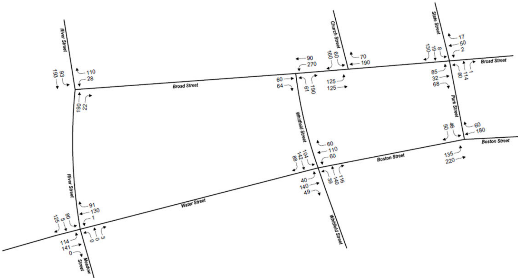
Figure 30 2029 No-Build Saturday Midday Peak Traffic Volumes
